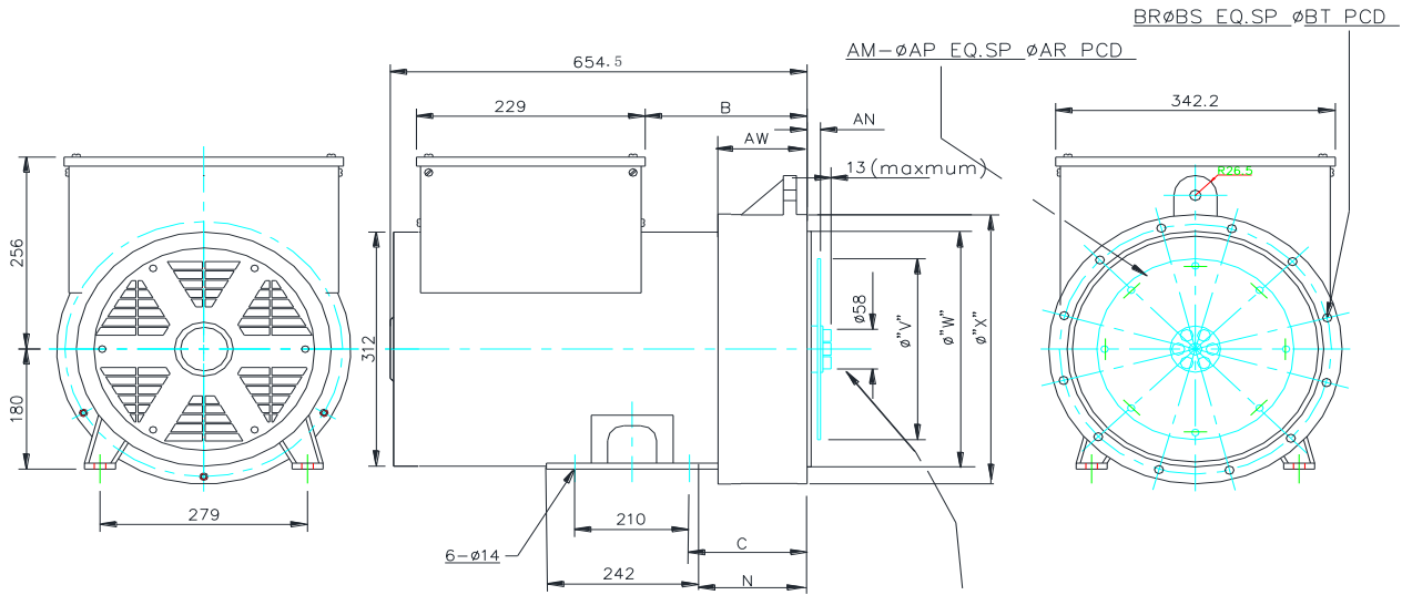
ADAPTOR
